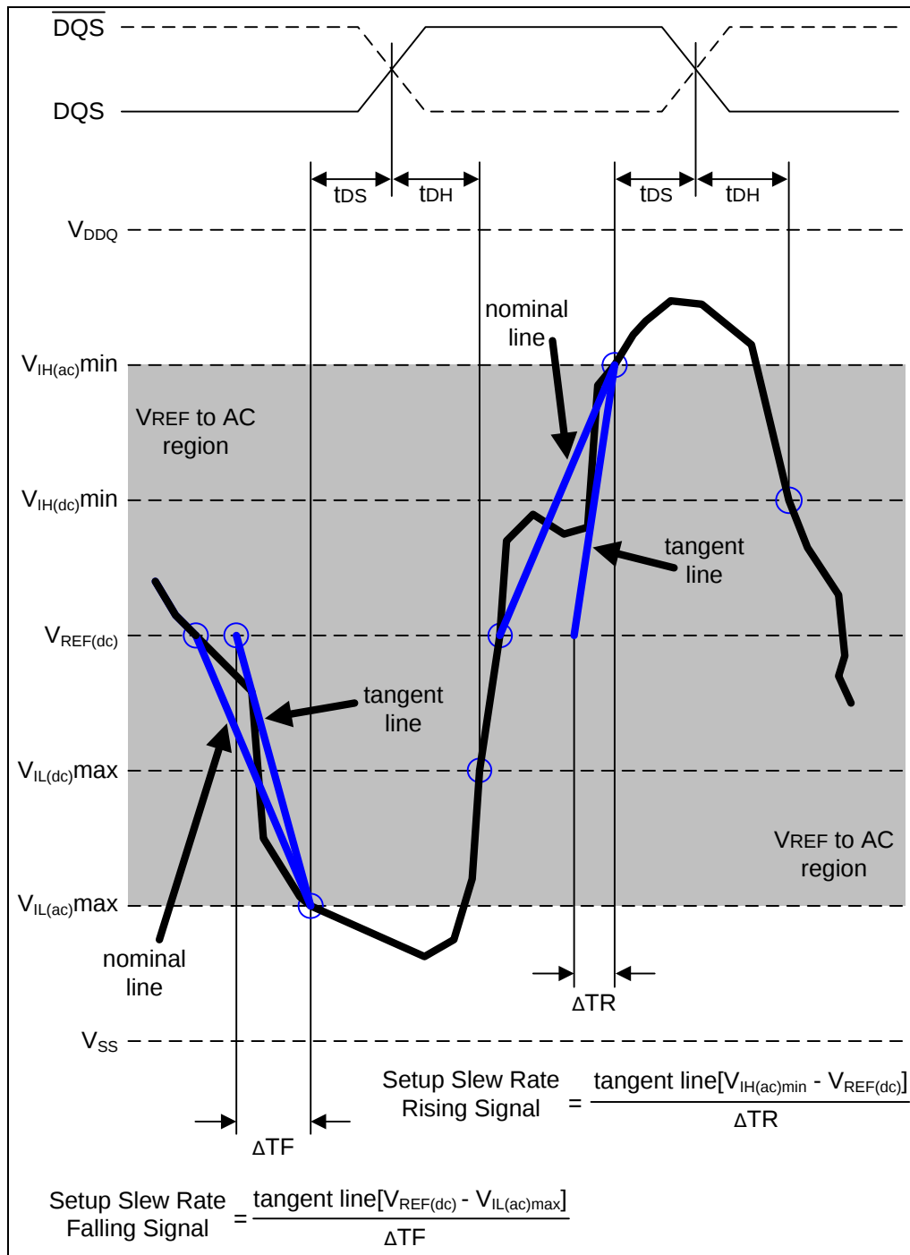
Figure 25 – Illustration of tangent line for t_{\text{DS}} (differential DQS, \overline{\text{DQS}} )
