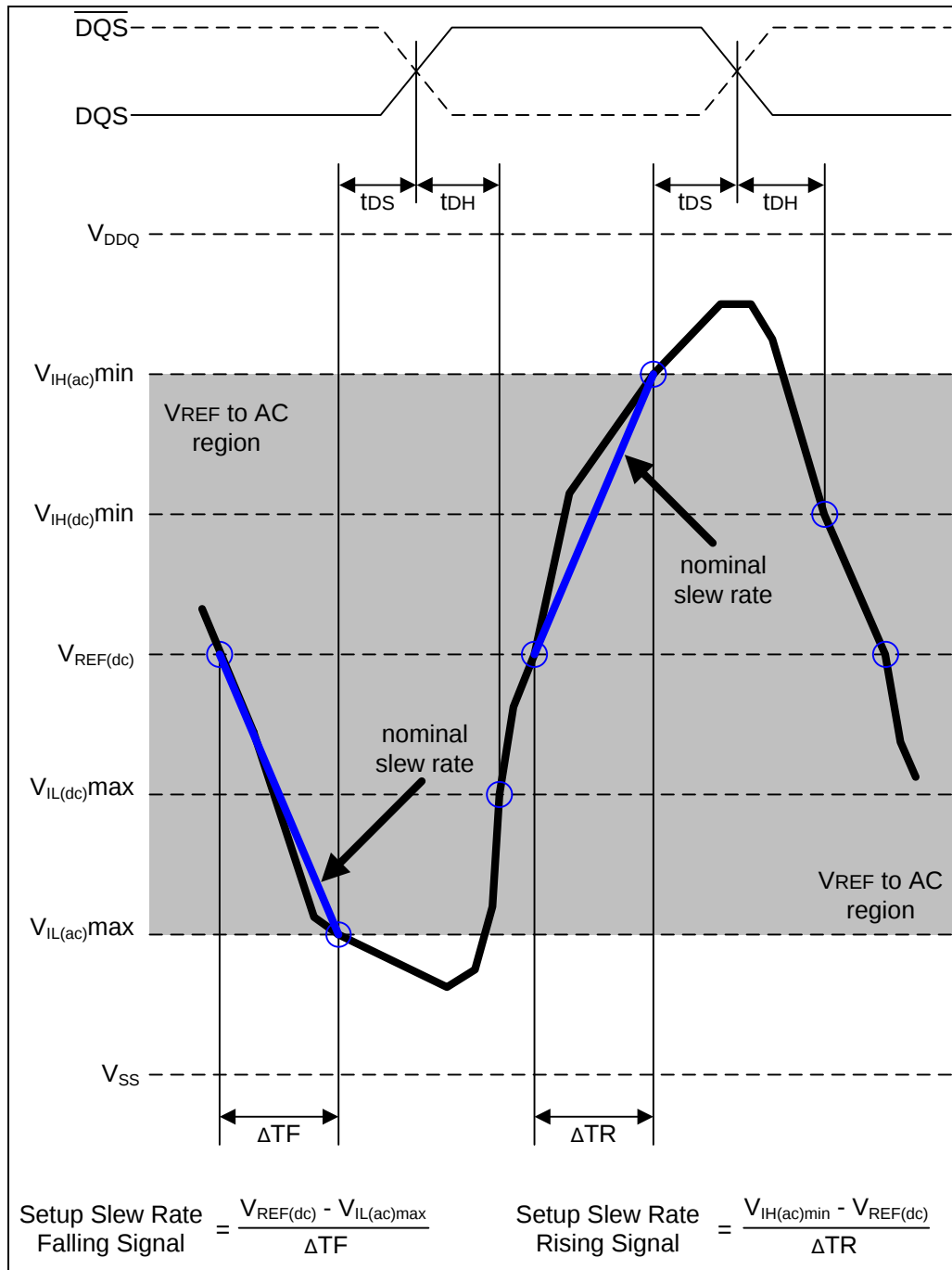
Figure 24 – Illustration of nominal slew rate for t_{DS} (differential DQS, \overline{\text{DQS}} )
